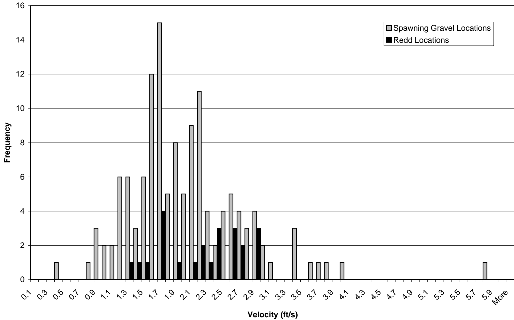
Figure 1. Velocity at Spawning gravel and Redd Locations on Butte Creek, March 2007. Velocity data were grouped into 0.1 ft/s bins.
